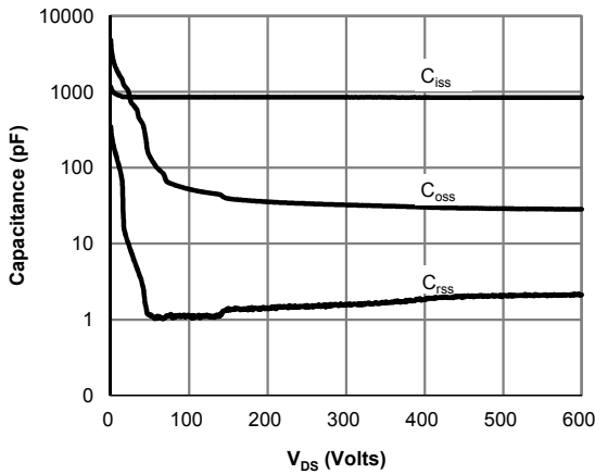
Figure 9: Capacitance Characteristics
