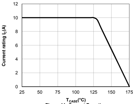
Figure 11: Current De-rating
