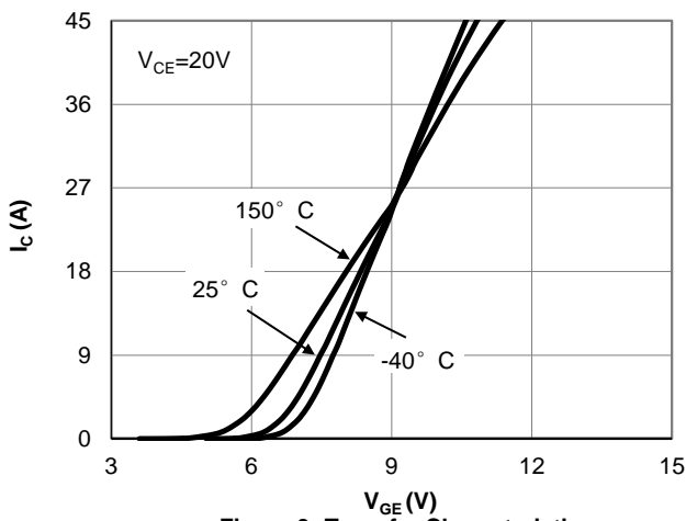
Figure 3: Transfer Characteristic
