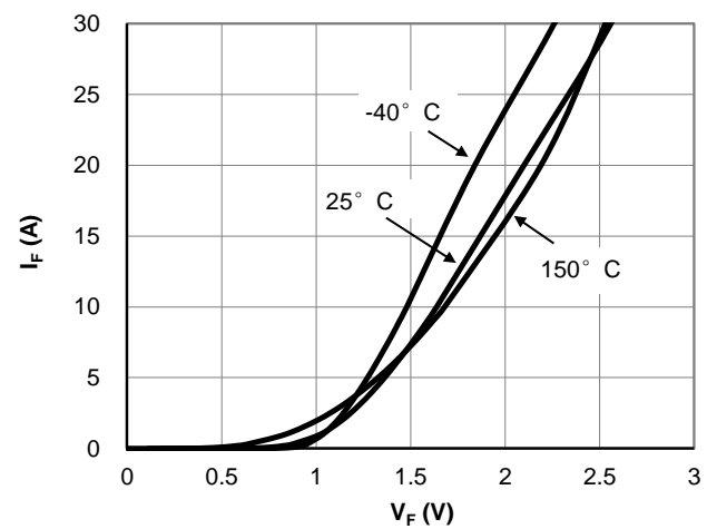
Figure 4: Diode Characteristic
