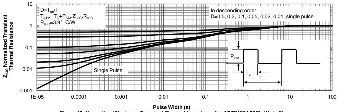
Figure 12: Normalized Maximum Transient Thermal Impedance for AOTF190A60CL (Note F)
