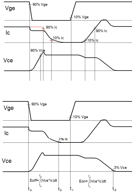
Figure B: Inductive Switching Test Circuit & Waveforms
