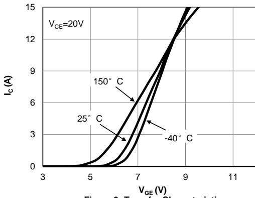
Figure 3: Transfer Characteristic
