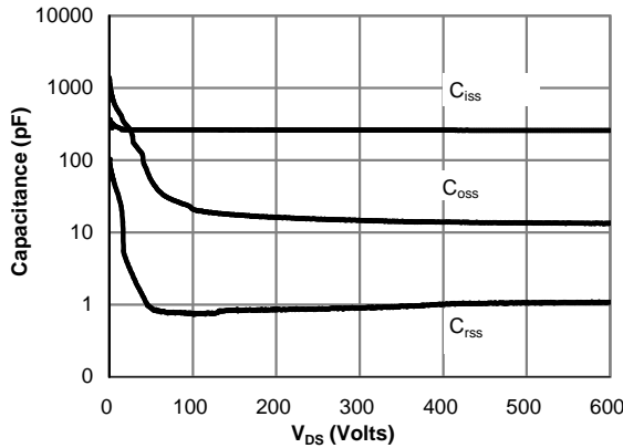
Figure 9: Capacitance Characteristics
