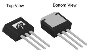
TO-262
