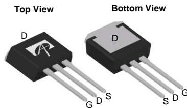
TO-262
