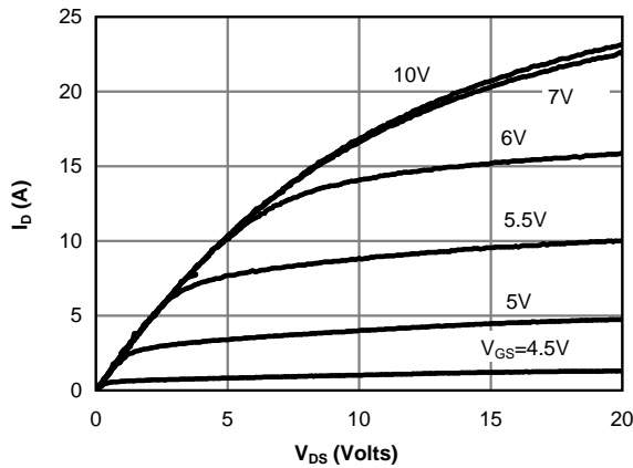
Figure 1: On-Region Characteristics @ 25°C
