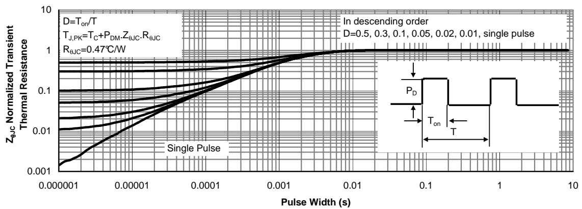
Figure 15: Normalized Maximum Transient Thermal Impedance for AOW20S60 (Note F)
