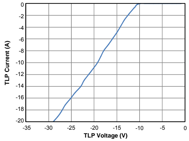
Negative TLP Clamping ( t_p = 100\text{ns} , t_r = 1\text{ns} )
