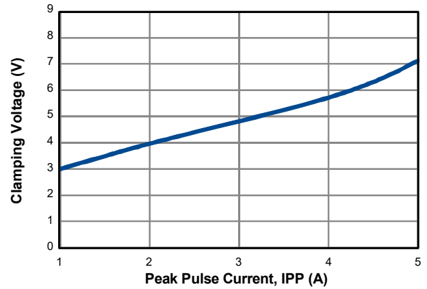
IEC61000-4-5 Surge 8/20 \mu\text{s} (I/O to GND and GND to I/O)
