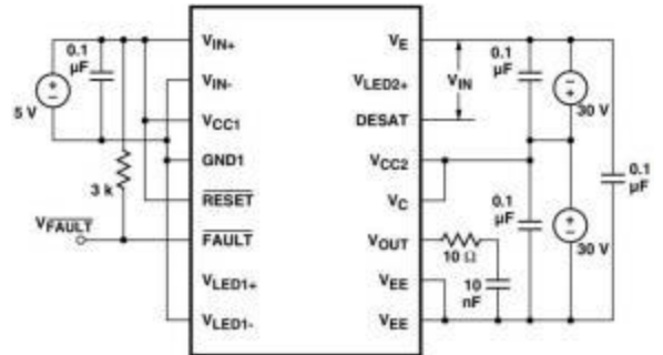
Figure 42. t_{DESAT(\overline{FAULT})} test circuit
