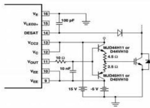
Figure 69. Current buffer for increased drive current
