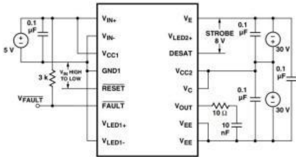
Figure 43. t_{RESET(FAULT)} test circuit.
