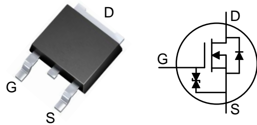
TO-252
