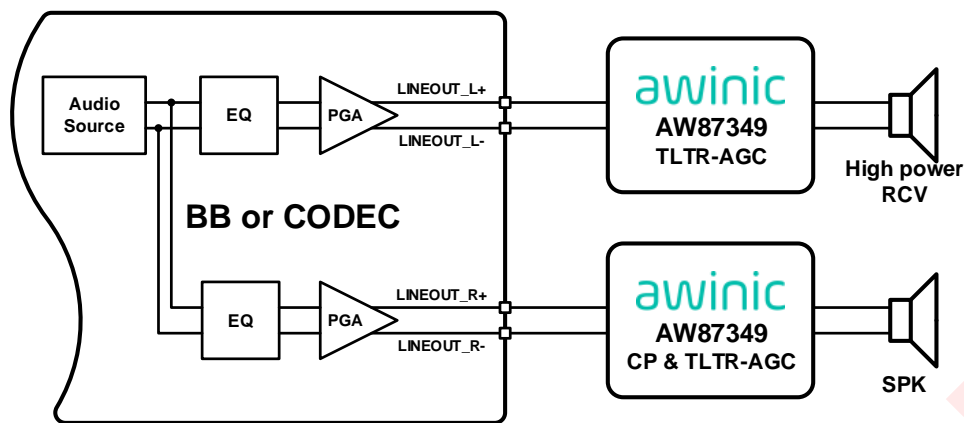
Figure 14 AW87349 High Power Receiver Stereo Mode Application
