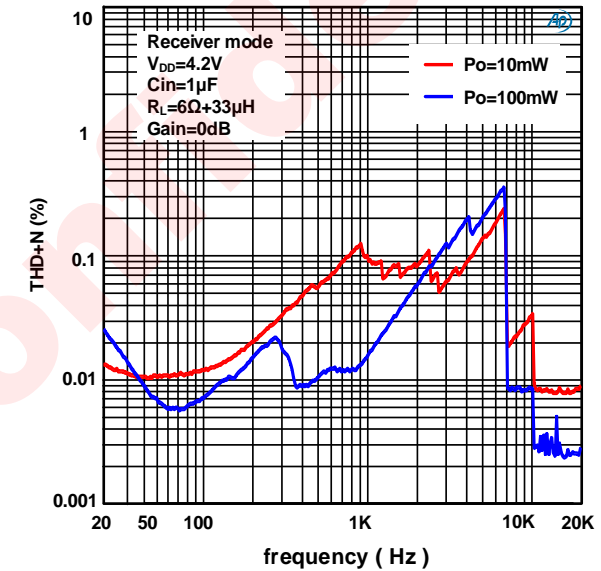
Class AB RCV THD+N vs frequency
