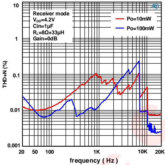
Class AB RCV THD+N vs frequency
