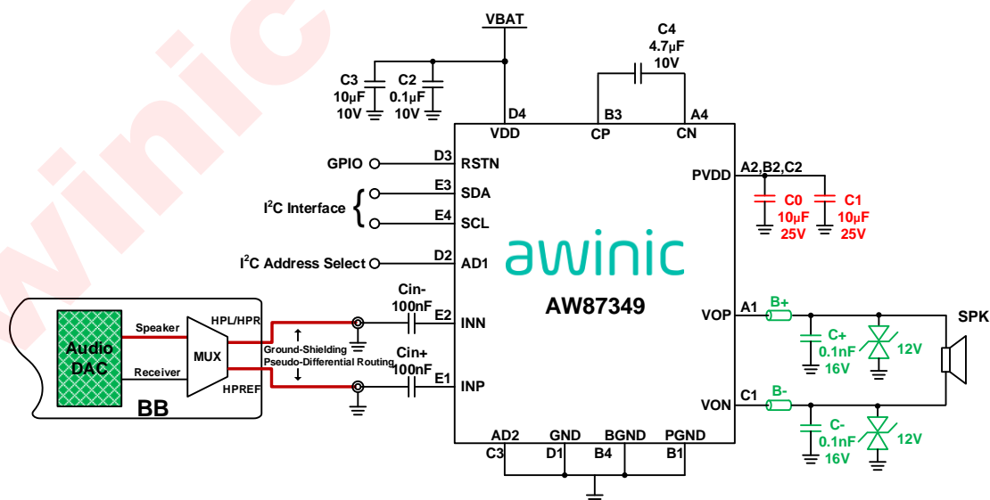
Figure 1 AW87349 Single-ended Input Mode Application Diagram
