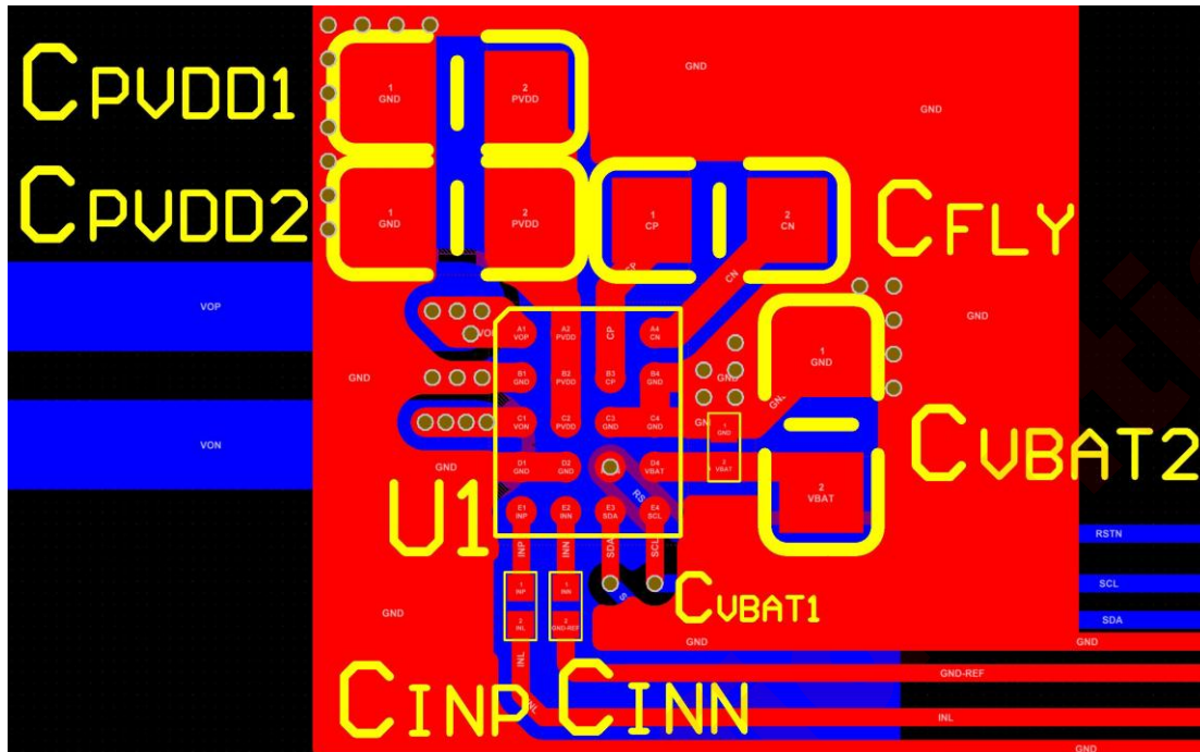
Figure 28 AW87349 Board Layout
