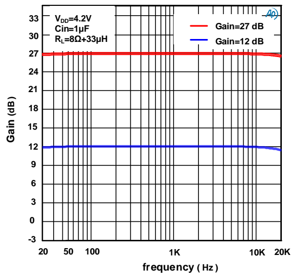
Class AB SPK Gain vs frequency
