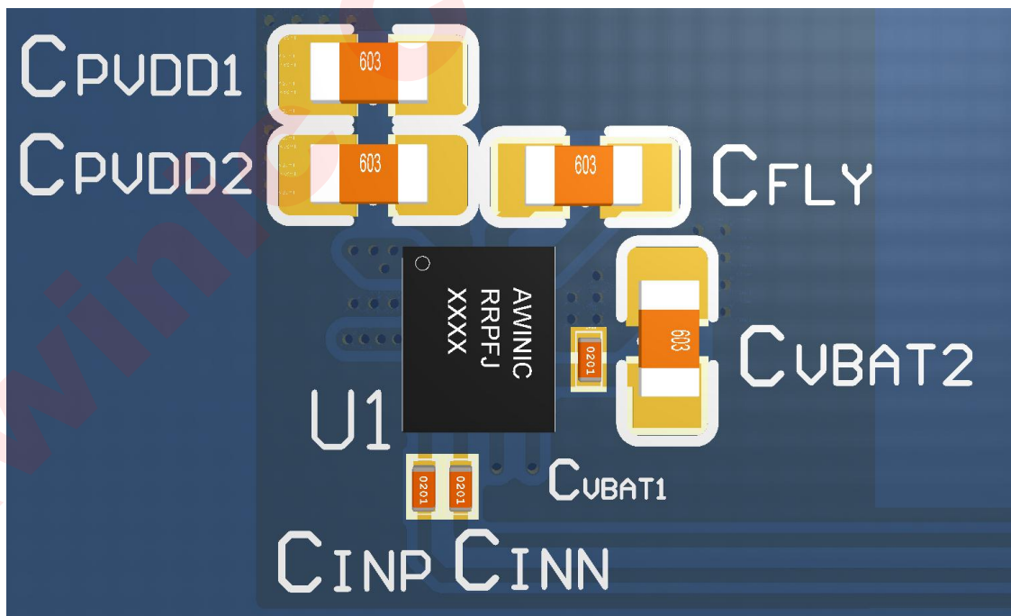
Figure 27 AW87349 External Components Placement
