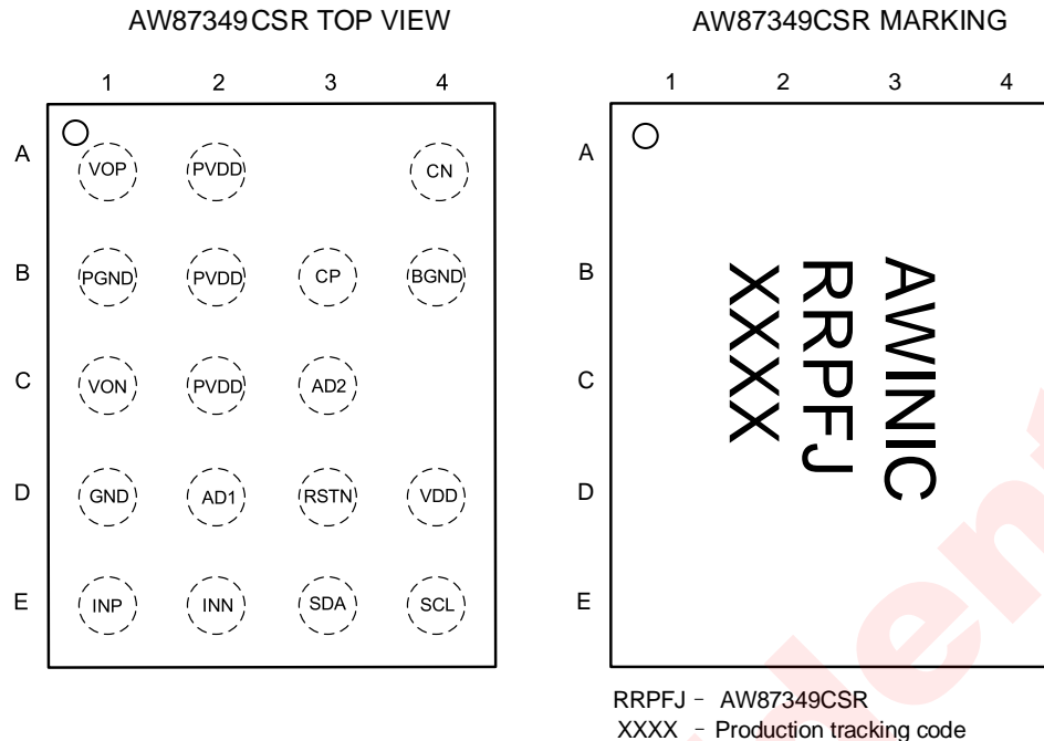
Figure 2 AW87349 Pin Diagram Top View and Device Marking
