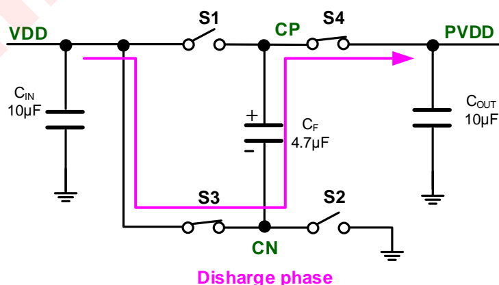
Figure 13 \Phi 2 : Flying Capacitor Charge is Transferred to C_{OUT}
