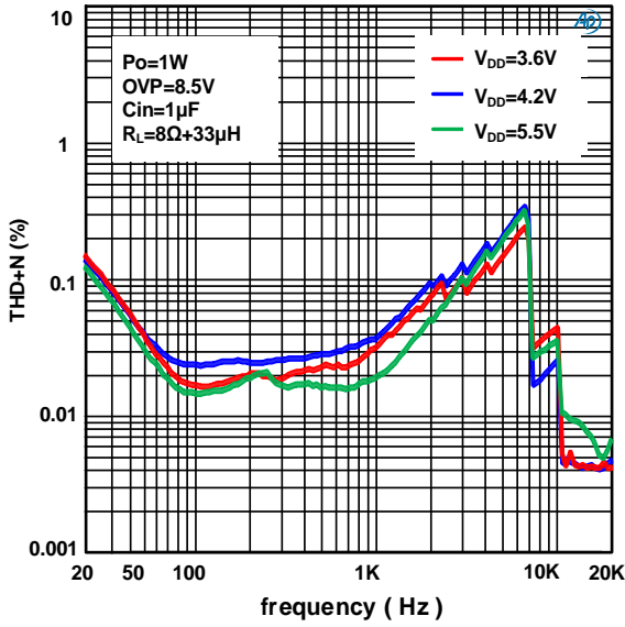
Class D THD+N vs frequency
