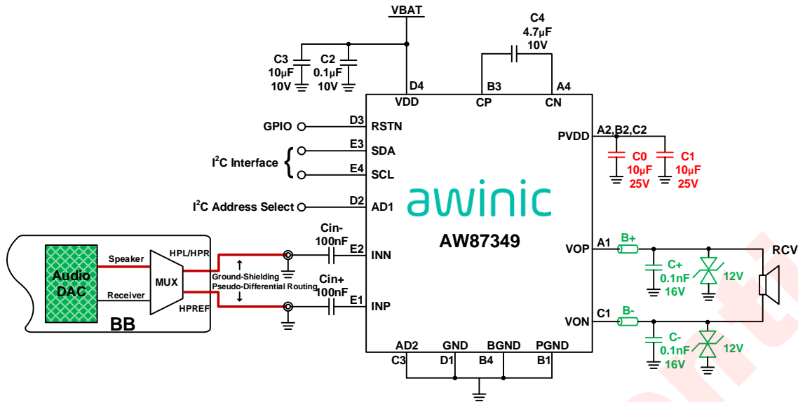
Figure 6 AW87349 High Power Receiver Stereo Mode Application
