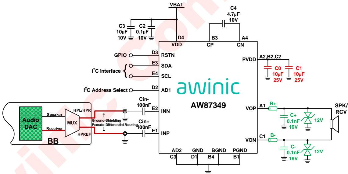
Figure 5 AW87349 Speaker &amp; Receiver 2-in-1 Mode Application Diagram
