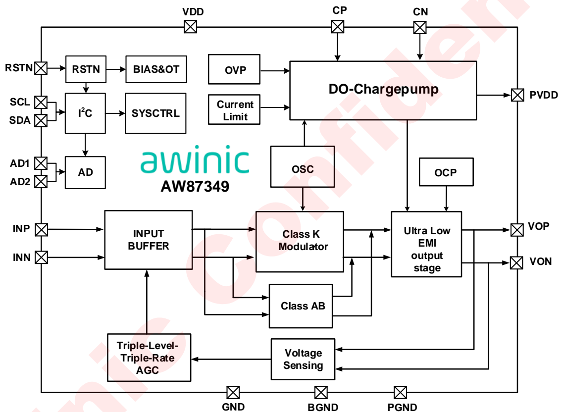
Figure 3 AW87349 Functional Diagram
