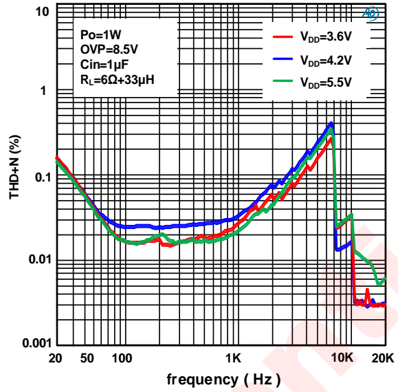
Class D THD+N vs frequency
