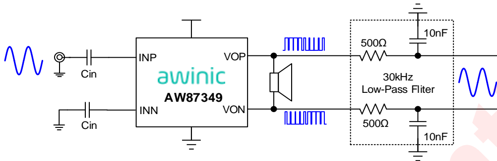
Figure 7 AW87349 Test Setup
