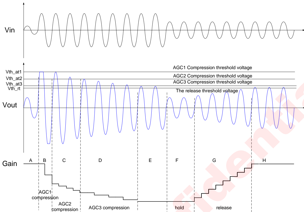
Figure 9 Triple-Level Triple-Rate AGC Operation Principle
