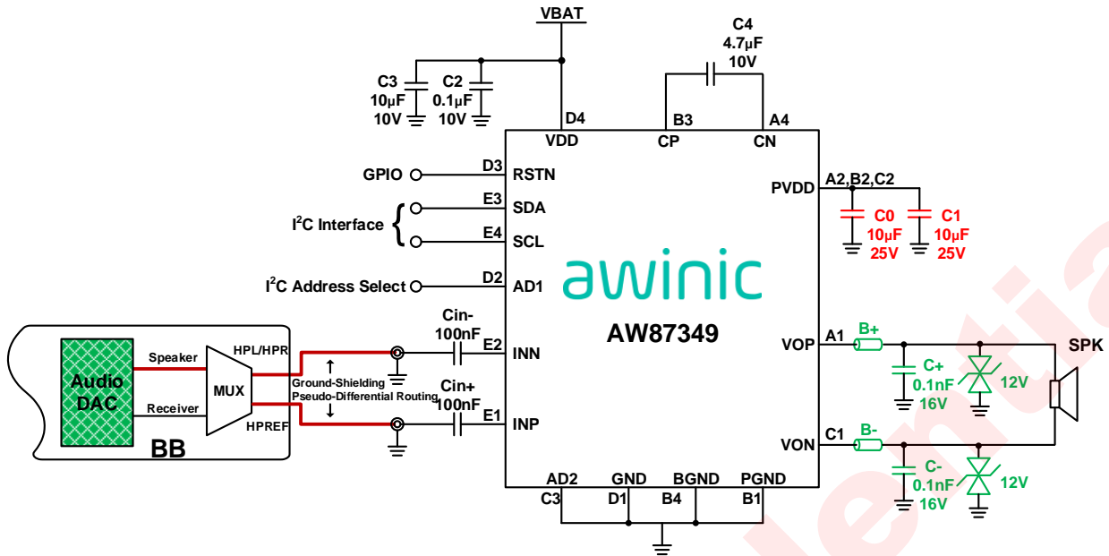
Figure 4 AW87349 Single-ended Input Mode Application Diagram (Note 1)
