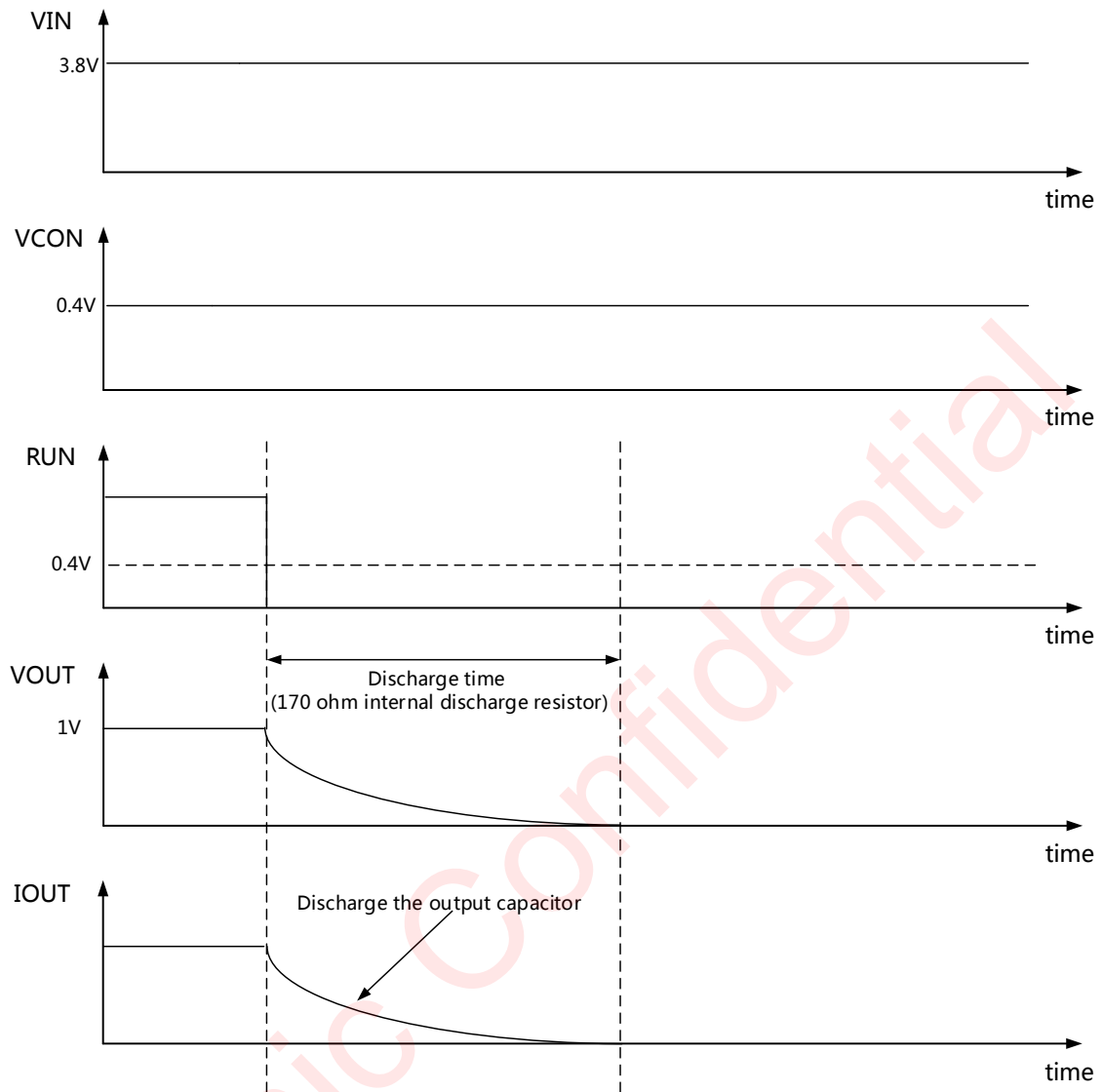
Figure 34 Power Off Sequence
