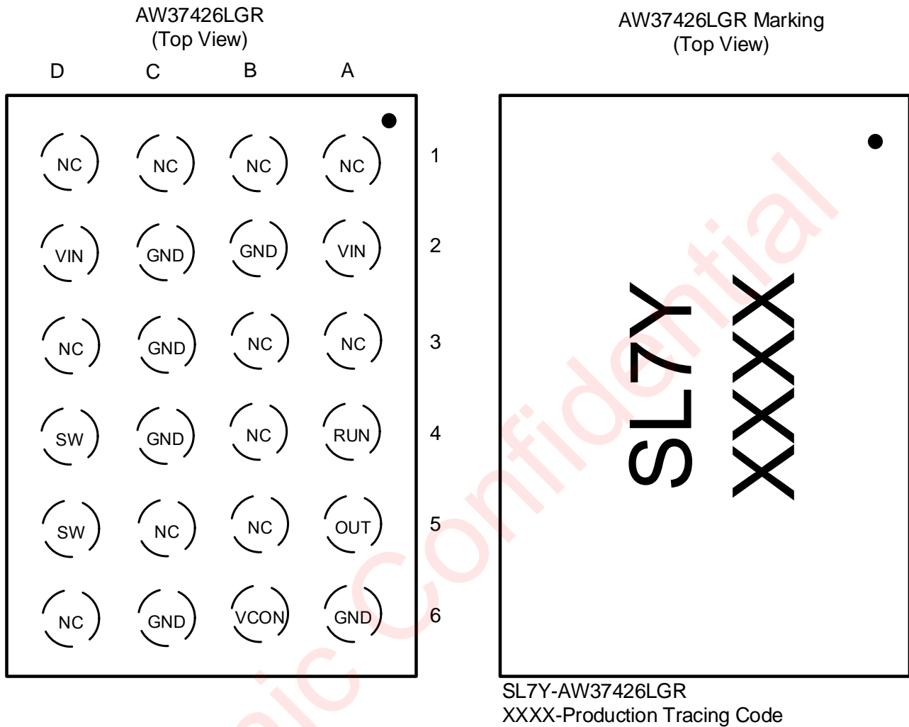
Figure 2 Pin Configuration and Top Mark
