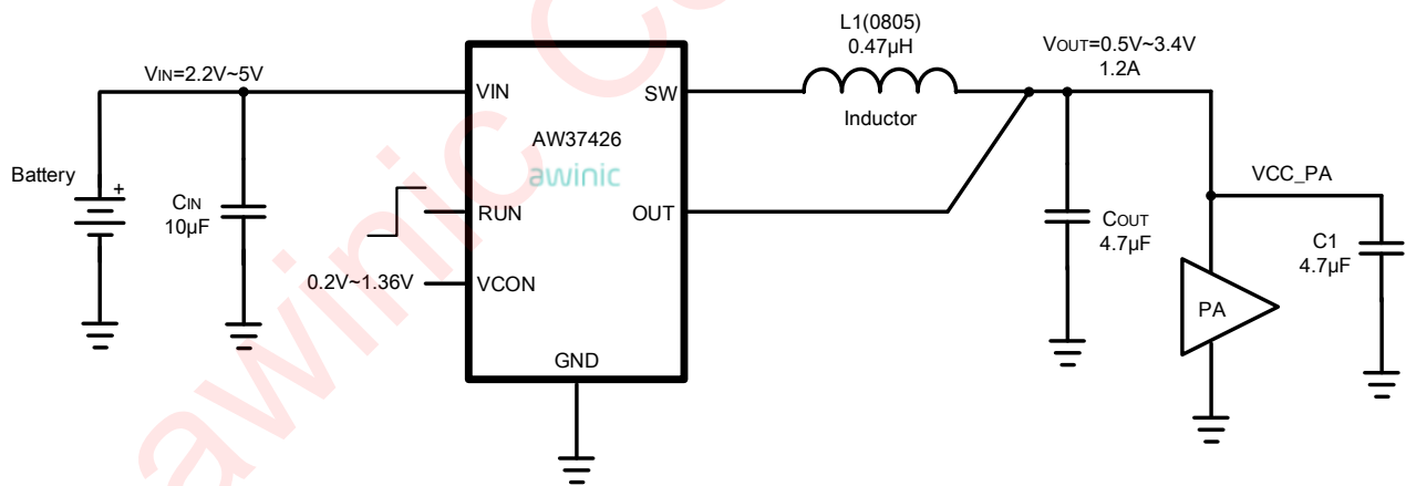
Figure 4 AW37426 Application Circuit
