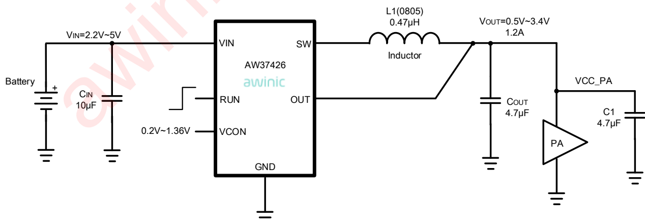
Figure 1 Typical Application Circuit of AW37426
