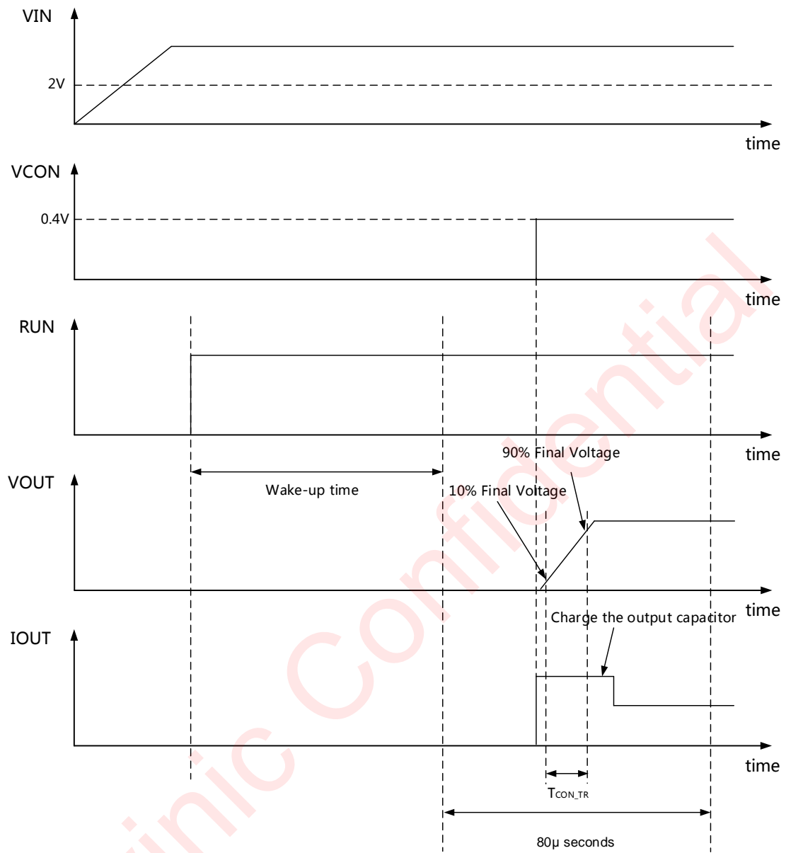
Figure 33 Power On Sequence
