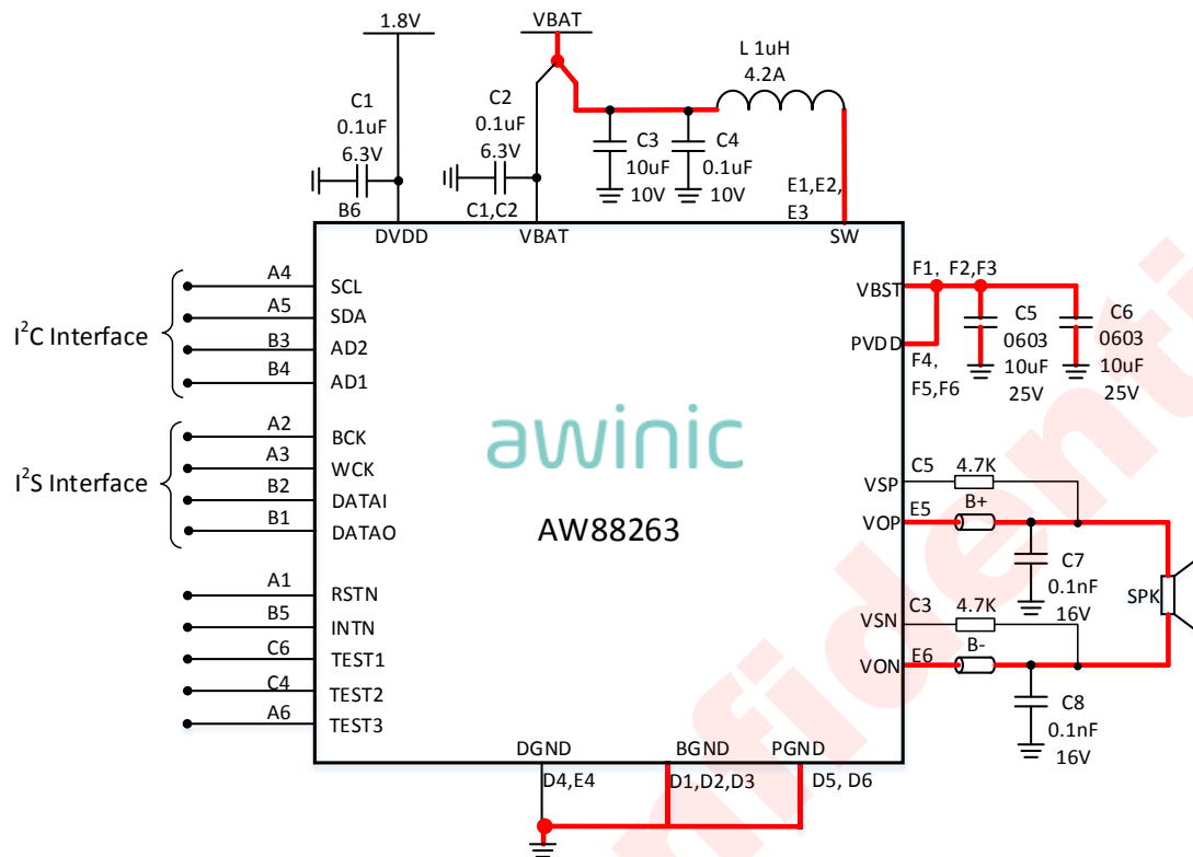
Figure 3 AW88263 Application Circuit
