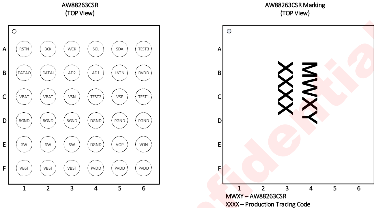
Figure 1 AW88263CSR pin diagram top view and device marking
