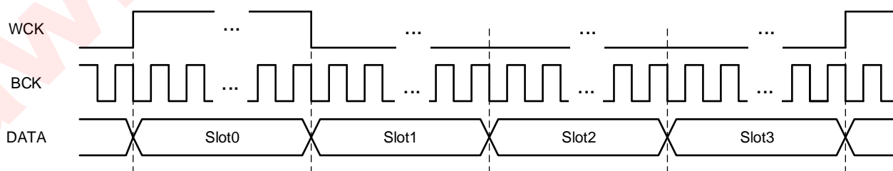
Figure 12 TDM Timing
