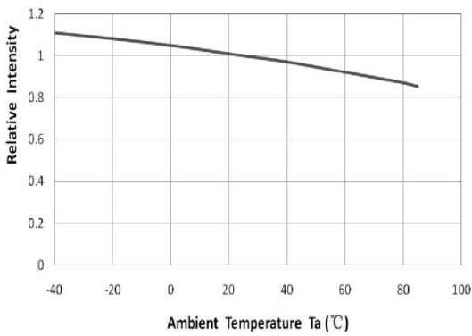
Relative Intensity VS. Ambient Temperature (Ta=25°C)
