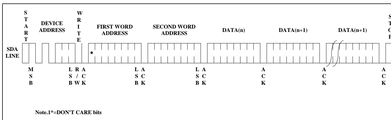
Figure 7. Page Write
