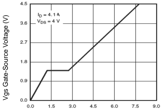
Qg Gate Charge (nC) Figure 11 Gate Charge
