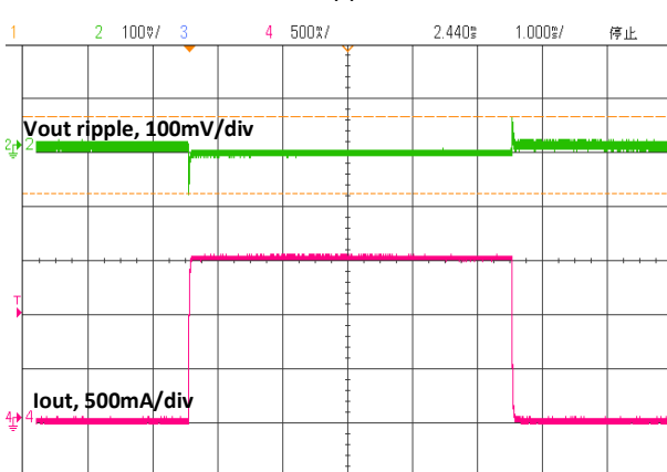
Load Transient
