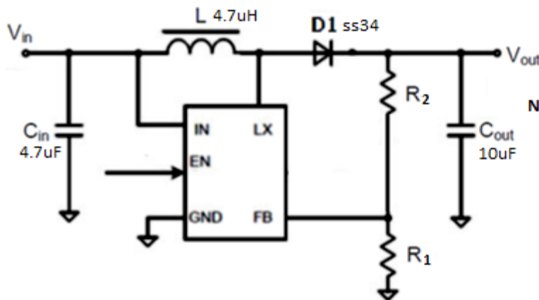
Figure1. BL8041 Typical Application Circuit
