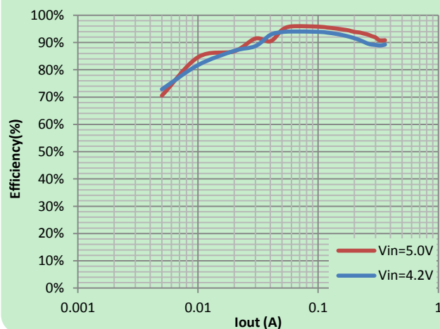
Efficiency Vout=12V
