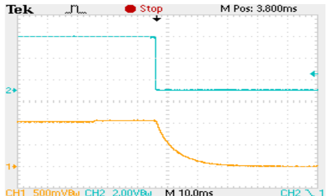
Shutdown Waveform
