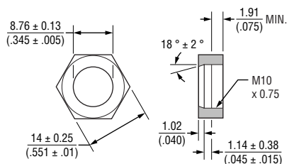
LOCKNUT H-38-10
