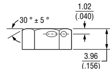
LOCKNUT H-38-4
