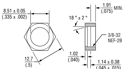
LOCKNUT H-38-4
