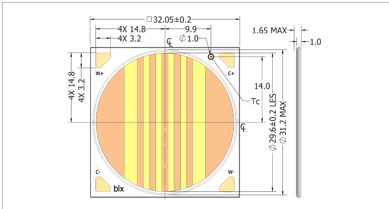
Figure 14: Drawing for Vesta Series Tunable White Gen 2 29mm Array
