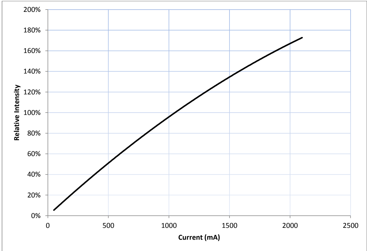
Figure 2: Typical Flux vs. Current, T_i = 25^\circ\text{C}
