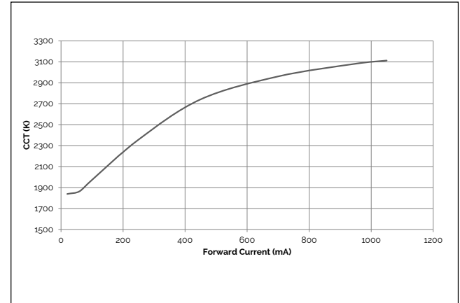
Figure 4: CCT vs. Forward Current
