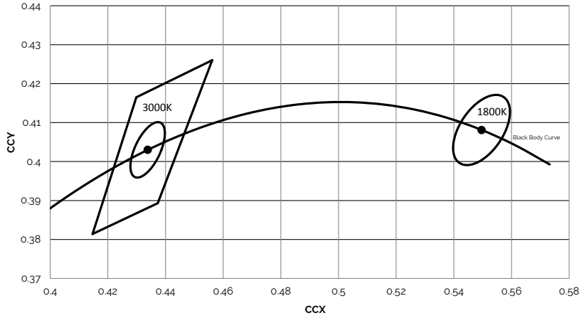
Figure 11: Graph of Warm White Test Bins in xy Color Space
