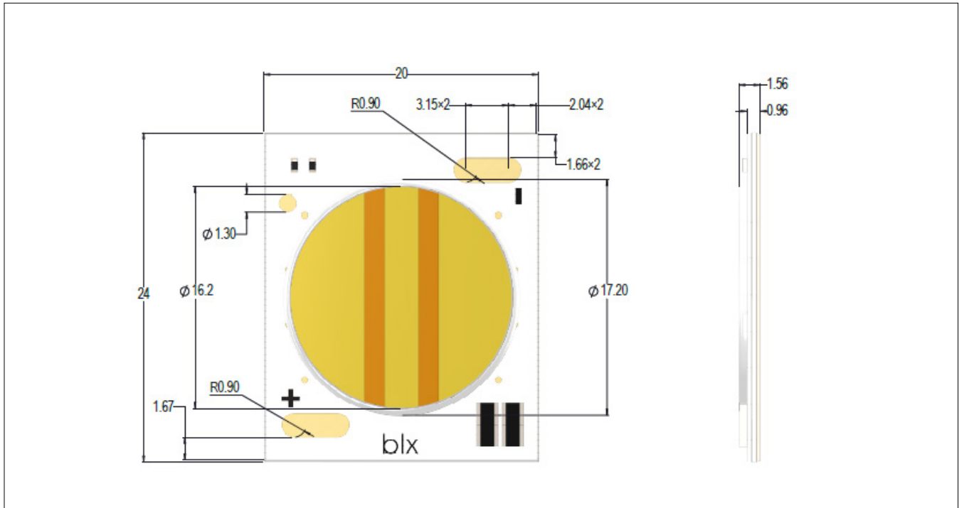
Figure 10: Drawing for Vesta Series Dim-To-Warm 15mm Array
