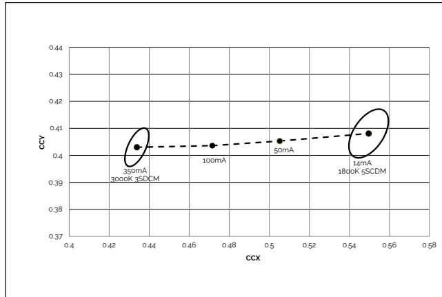
Figure 5: Color Shift vs. Forward Current
