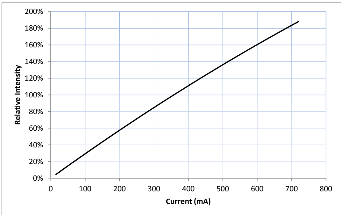
Figure 2: Typical Flux vs. Current, T_j = 25^\circ\text{C}
