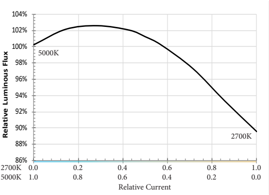
Figure 8: Derating Curve
