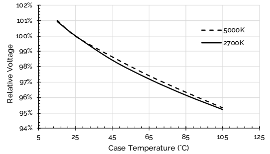
Figure 4: Forward Voltage vs. Case Temperature
