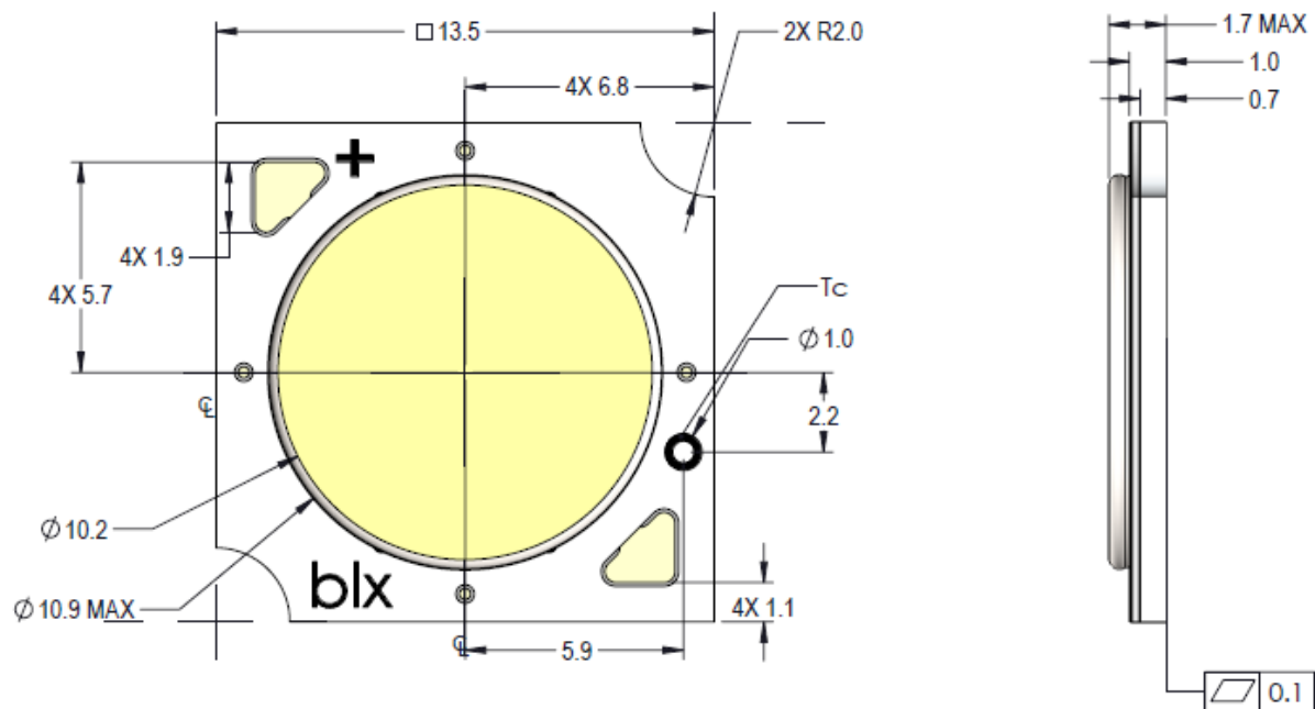
Figure 18: Drawing for V10 LED Array
