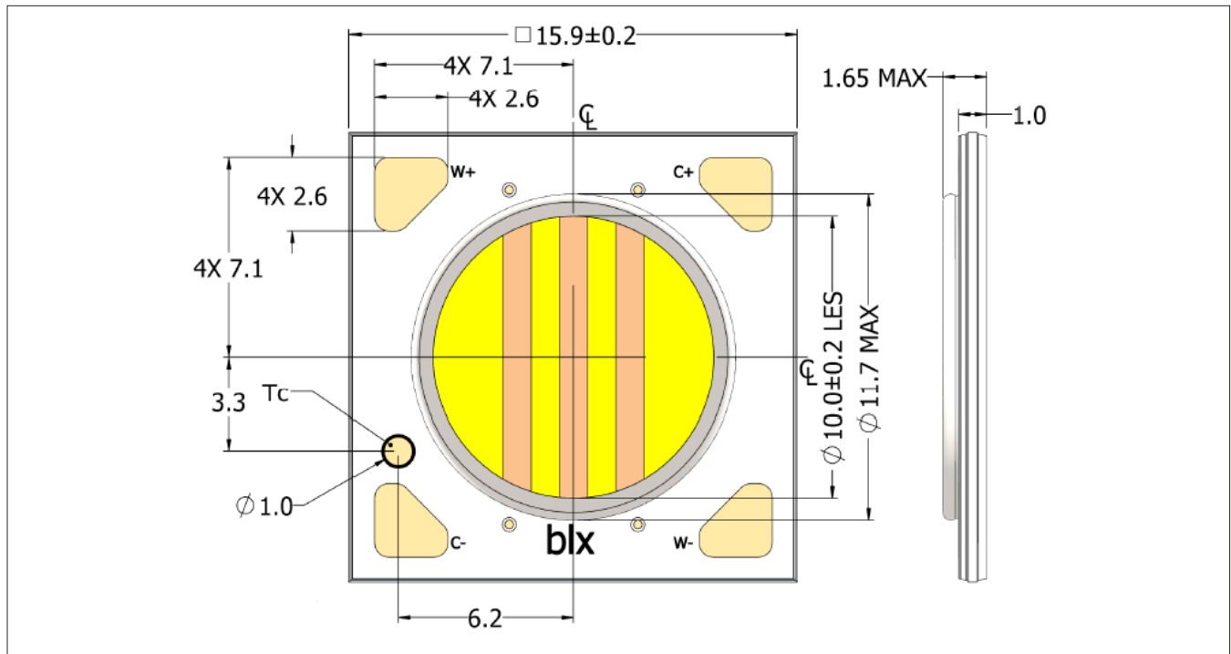
Figure 14: Drawing for Vesta Series Tunable White Gen2 gmm Array
