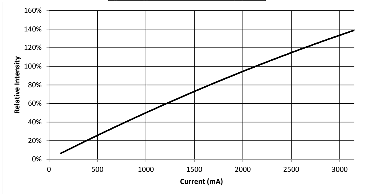
Figure 3: Typical Flux vs. Drive Current, Tj = 25°C
