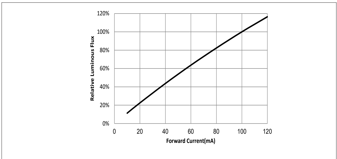
Figure 4: Typical Relative Luminous Flux vs. Drive Current ( T_{sp}=25^{\circ}\text{C} )
