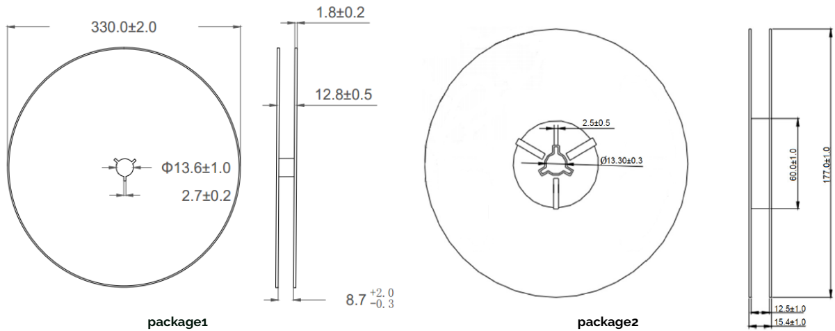
Figure 14: Emitter Reel Drawings
