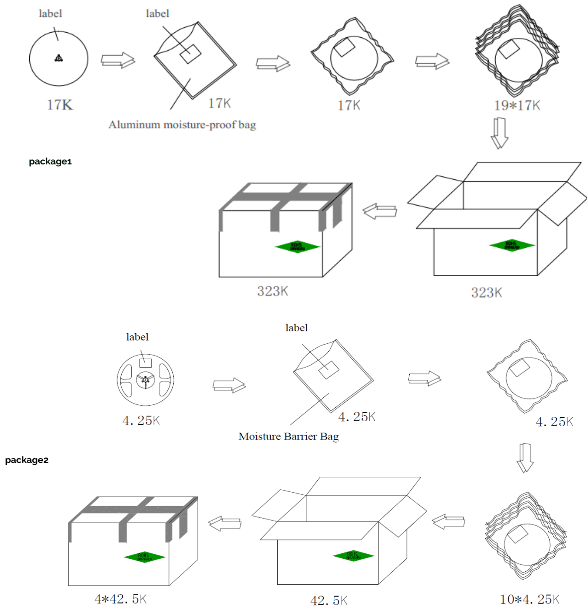
Figure 16: Emitter Reel Packaging Drawings
