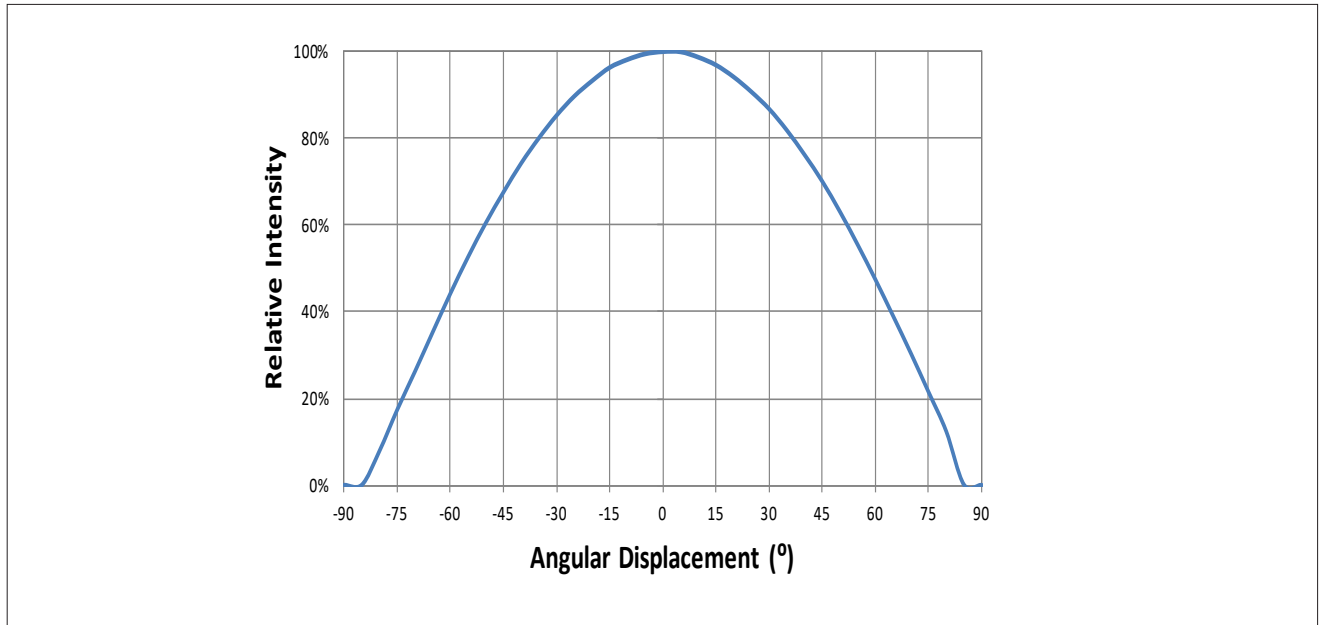
Figure 8: Typical Spatial Radiation Pattern at 100mA, T_{sp} = 25^{\circ}\text{C}
