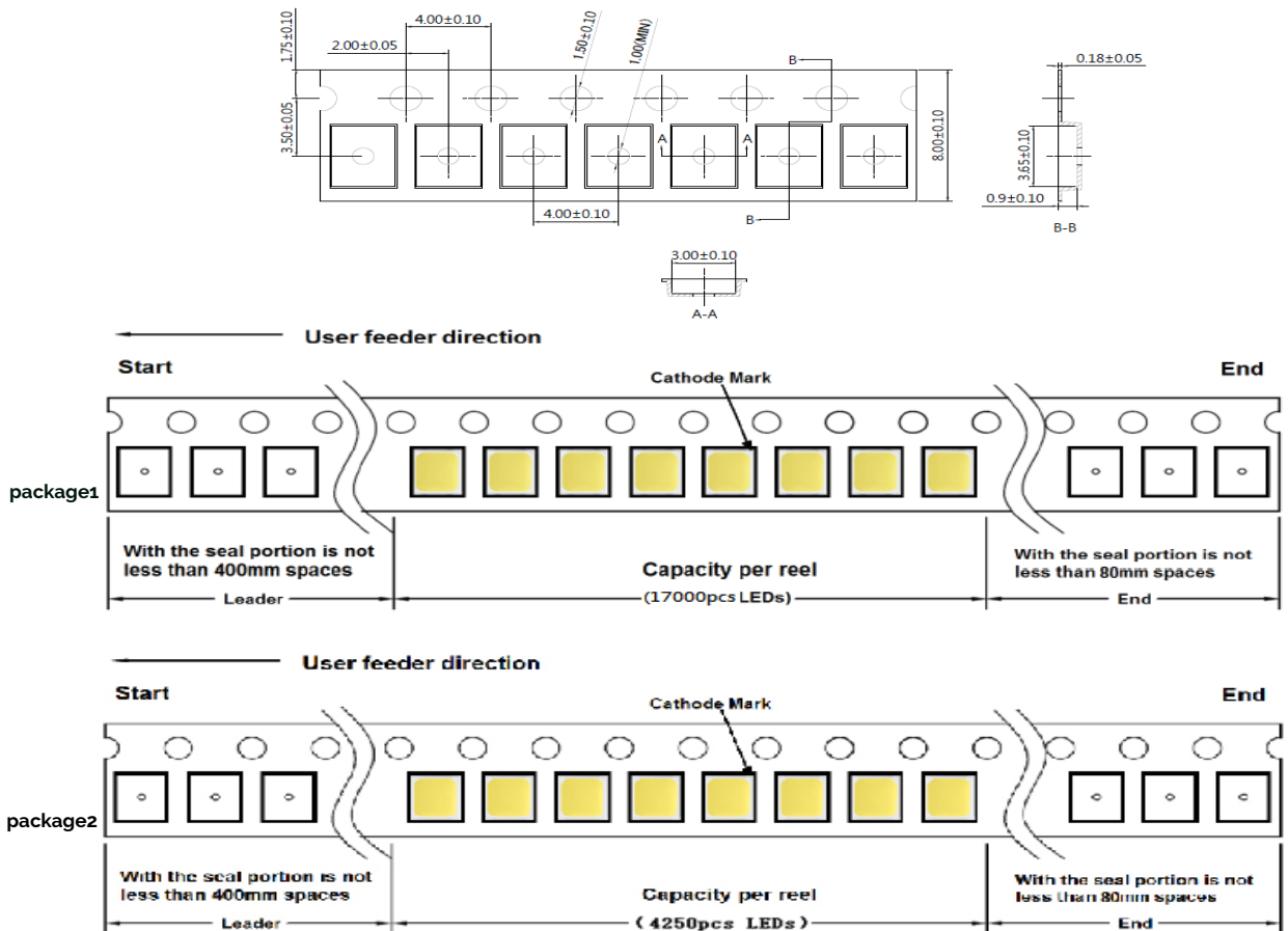
Figure 15: Emitter Tape Drawings
