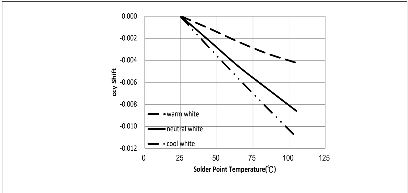
Figure 7: Typical ccy Shift vs. Solder Point Temperature
