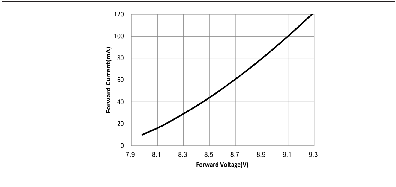
Figure 3: Drive Current vs. Voltage ( T_{sp}=25^{\circ}\text{C} )
