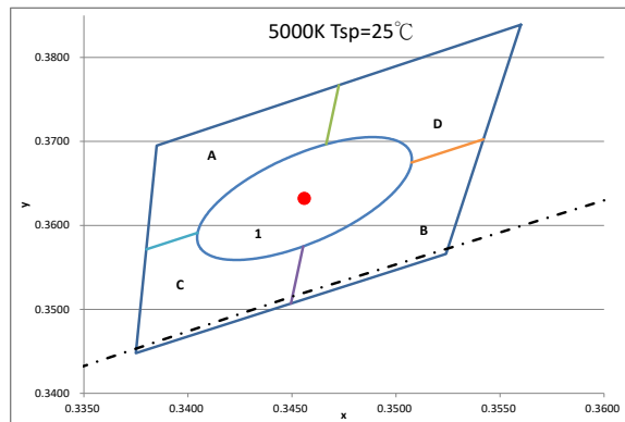
Figure 2: C.I.E. 1931 Chromaticity Diagram (5 Color Bin Structure, Hot-color Targeted at T_{sp}=85^{\circ}\text{C} , 5000K/6300K at T_{sp}=25^{\circ}\text{C} )
