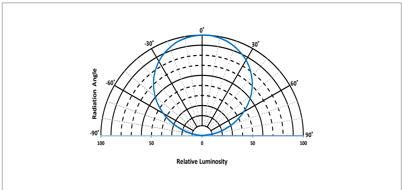
Figure 9: Typical Polar Radiation Pattern at 100mA, T_{sp} = 25^{\circ}\text{C}
