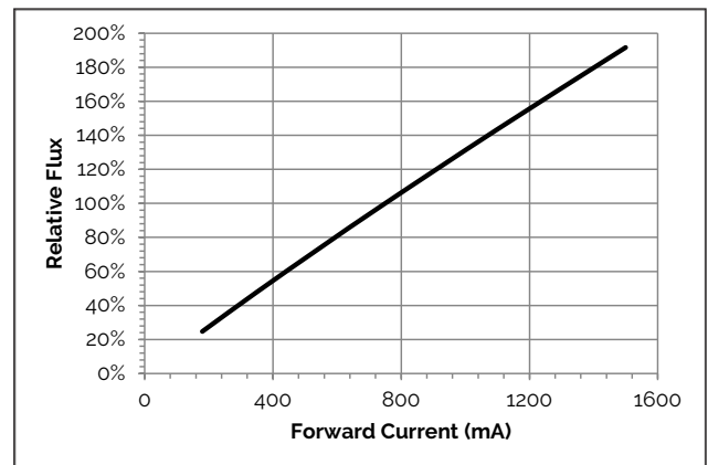
Figure 4: Flux vs. Current (560mm only)
