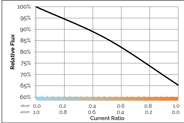
Figure 13: Flux vs. Current Ratio (1800K-4000K)
