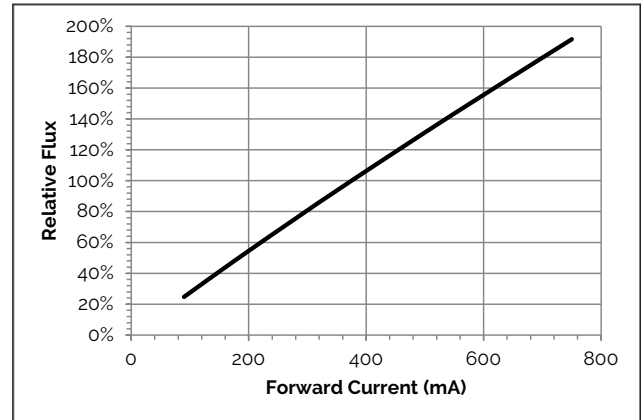
Figure 2: Flux vs. Current (280mm only)
