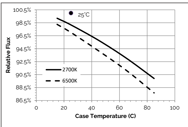
Figure 17: Flux vs Case Temperature (2700K-6500K)
