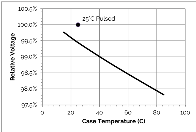
Figure 15: Voltage vs Case Temperature
