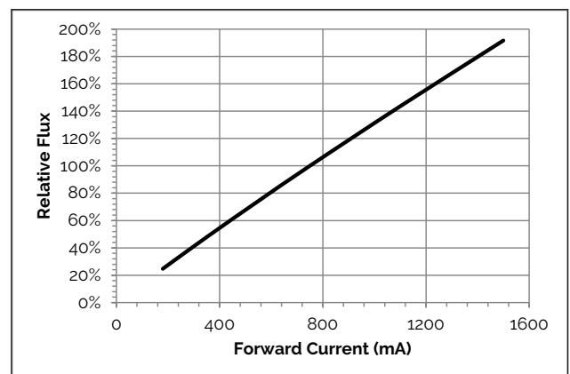
Figure 6: Flux vs. Current (1120mm only)
