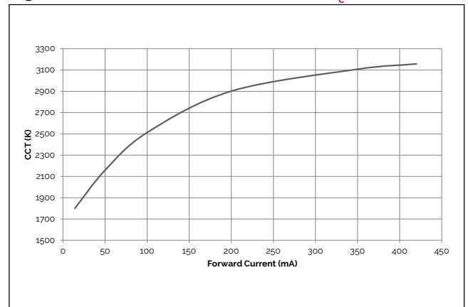
Figure 6: 12W CCT vs. Forward Current, T_c=25^\circ\text{C}
