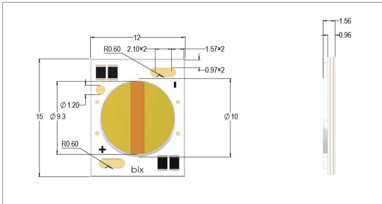
Figure 13: Drawing for Vesta™ Dim-To-Warm gmm Array
