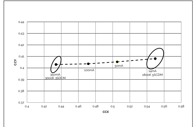
Figure 8: Color shift vs. Forward Current
