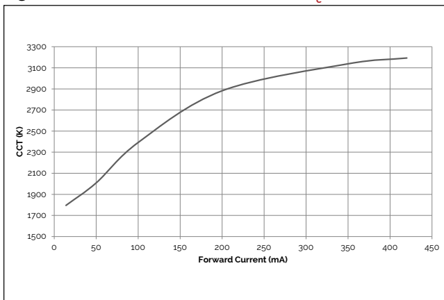
Figure 5: 6W CCT vs. Forward Current, T_c=25^\circ\text{C}
