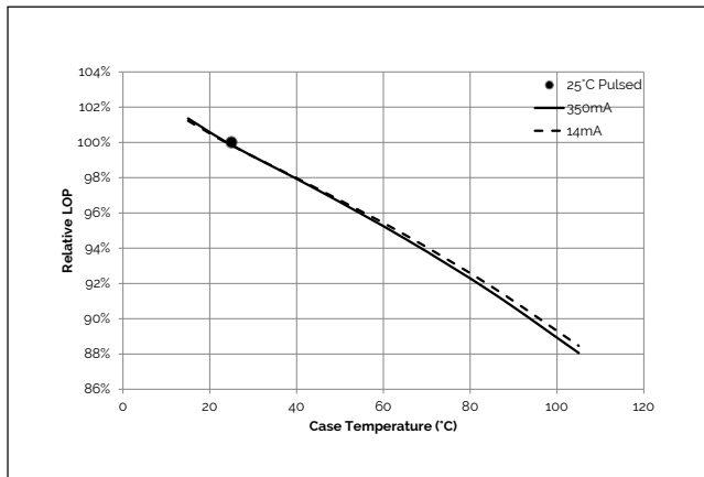
Figure 3: 6W Relative Flux vs. Case Temperature
