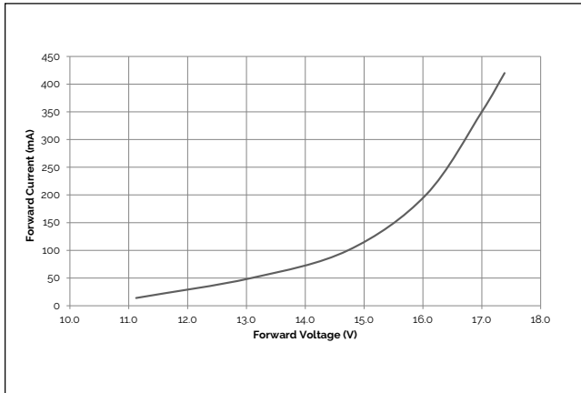
Figure 1: 6W Forward Voltage vs. Forward Current, T_c=25^\circ\text{C}
