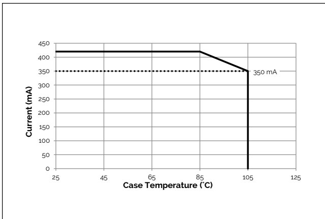
Figure 9: Derating Curve
