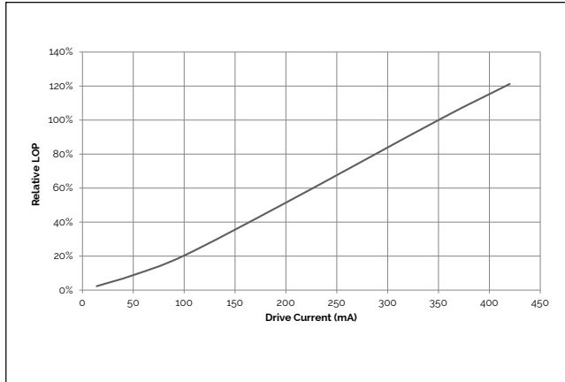
Figure 7: Relative LOP vs. Drive Current, T_c=25^\circ\text{C}
