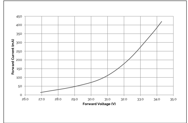
Figure 2: 12W Forward Voltage vs. Forward Current, T_c=25^\circ\text{C}
