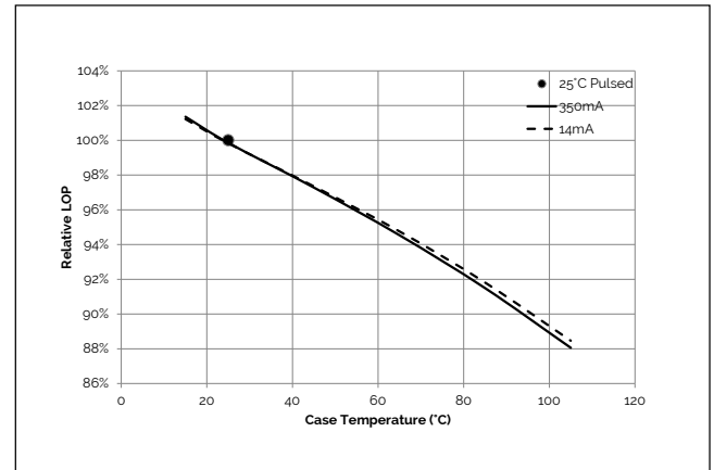
Figure 4: 12W Relative Flux vs. Case Temperature
