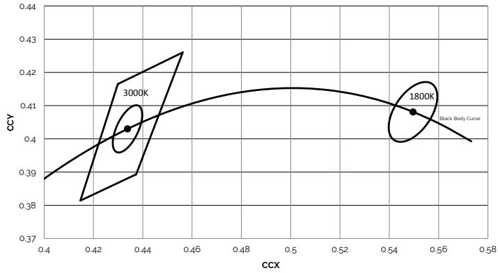
Figure 14: Graph of Warm White Test Bins in xy Color Space
