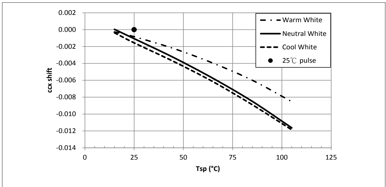
Figure 5: Typical DC cxx Shift vs. Solder Point Temperature
