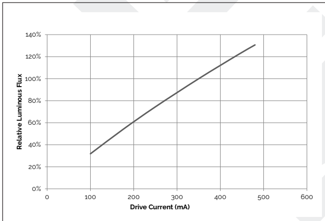
Figure 12: Typical Relative Flux vs. Current V6B HD 1,2
