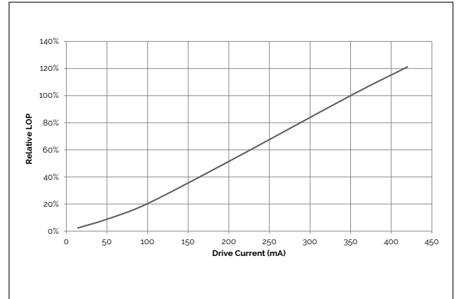
Figure 10: 12W Relative LOP vs. Drive Current, T_c=25^\circ\text{C}
