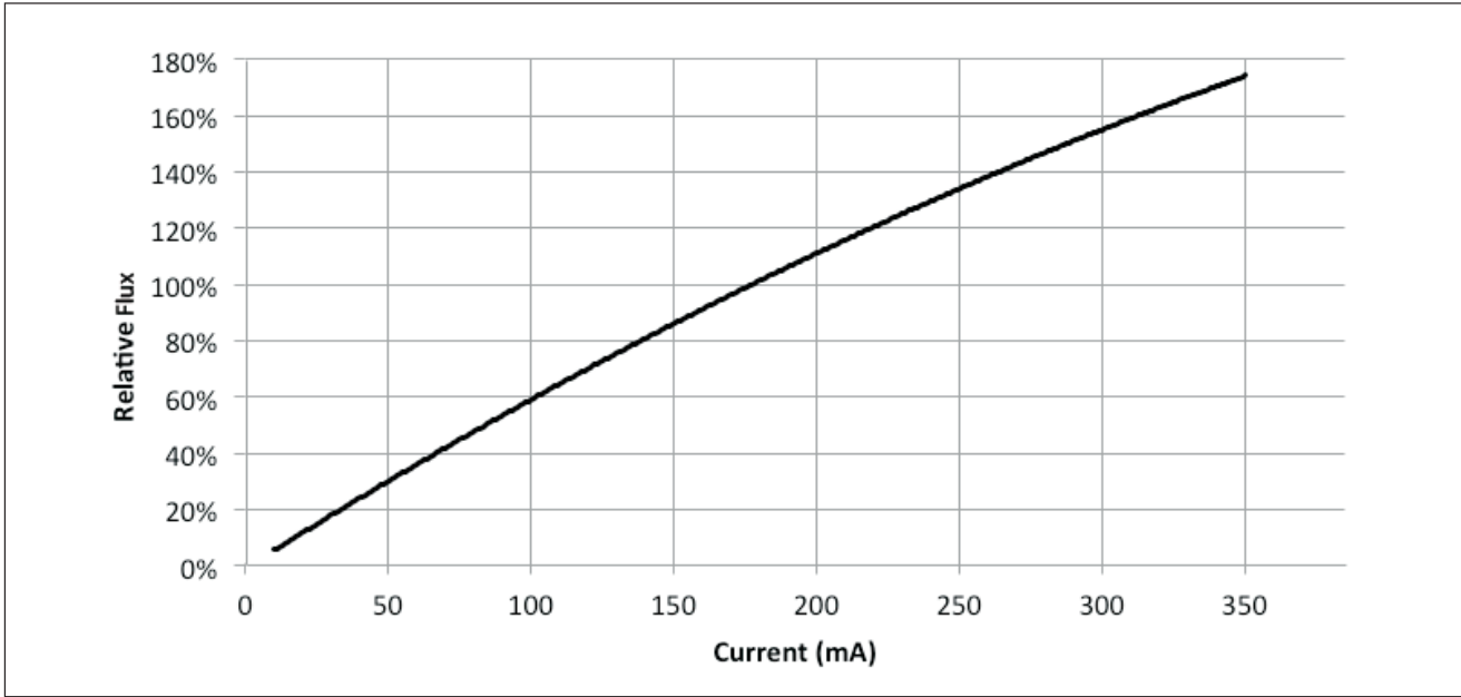
Figure 3: Typical Relative Luminous Flux vs. Current – BXRE-xxx0800-A-2x
