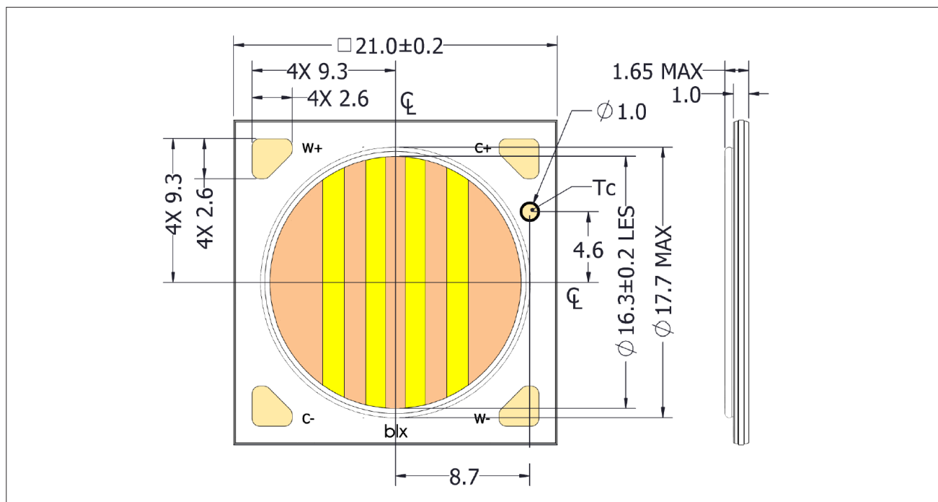
Figure 14: Drawing for Vesta Series Tunable White Gen 2 15mm Array
