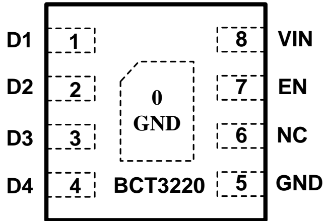
DFN2x2-8L Package
