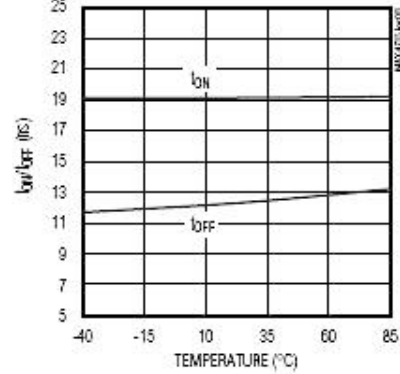
TURN-ON/OFF TIME vs. TEMPERATURE
