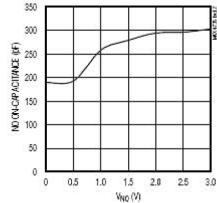
NO_ ON-CAPACITANCE vs. NO_ VOLTAGE
