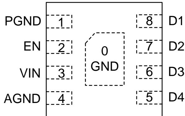
DFN2x2-8L
