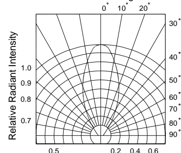
FIG.8 Radiant Diagram
