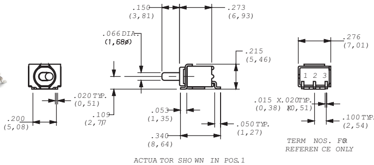
GT11MSABE Horizontal Actuation SPDT
