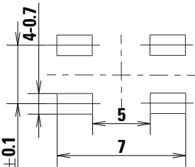
PCB LAND DIMENSION
