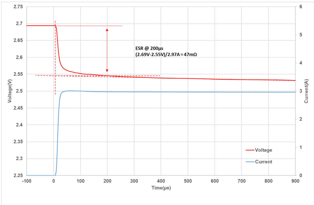
Fig 2: GY12R708020S335R-L ESR Measurement
