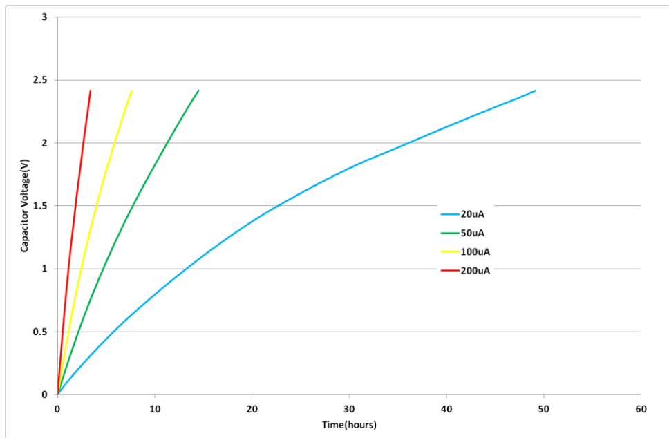
Fig 11: Charging an HA130 with low current
