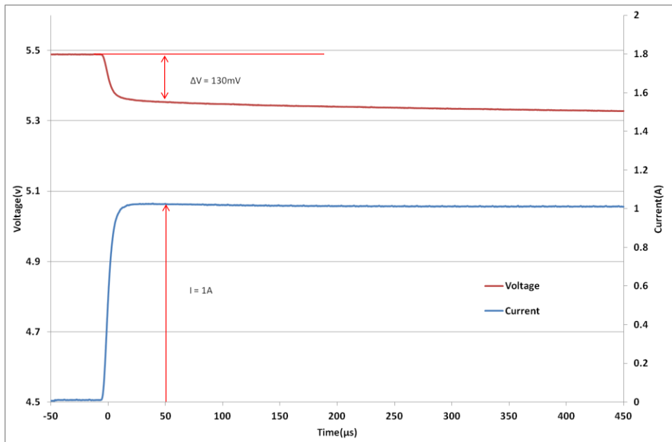
Fig 3: Measurement of ESR for an HA230
